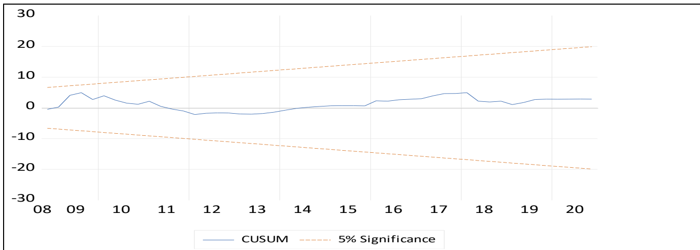
Figure 1: CUSUM Stability Test
